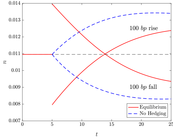
Figure 1: Impulse response of bank net worth to a 100 bp change in interest rates, with and without dynamic hedging.
